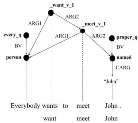
Figure 5: Semantic representation of the sentence “Everybody wants to meet John” from Buys and Blunsom (2017). The graph is based on the Elementary Dependency Structure (EDS) representation of Minimal Recursion Semantics (MRS). The alignments are given together with the corresponding tokens, and lemmas of surface predicates and constants.
