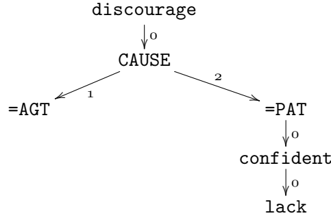
Figure 18: The definition of discourage in the 4lang concept lexicon exemplifies the use of ‘cause’ in associative network representations of linguistics knowledge. The graph expresses that discourage means, that the agent (=AGT) causes the participant that is called patient in linguistics (=PAT) to lack confidence.
