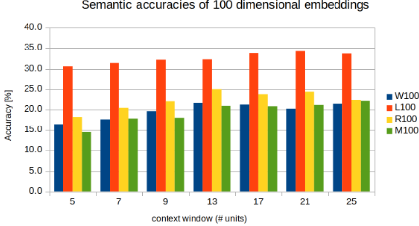
Figure 9: Semantic accuracy of Hungarian 100 dimensional embeddings with different strategies.
