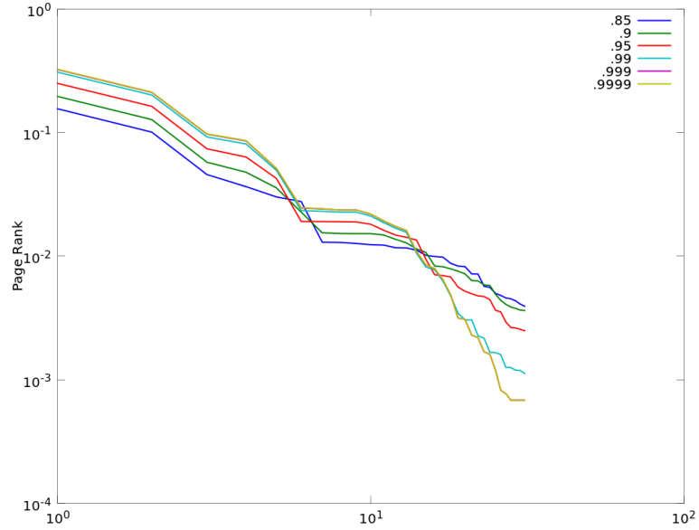
Figure 7: PageRank of concepts. Concepts are sorted by PageRank. If the n th concept has PageRank p , it is shown at x = \log n , y = \log p . Colors correspond to different damping factors.
