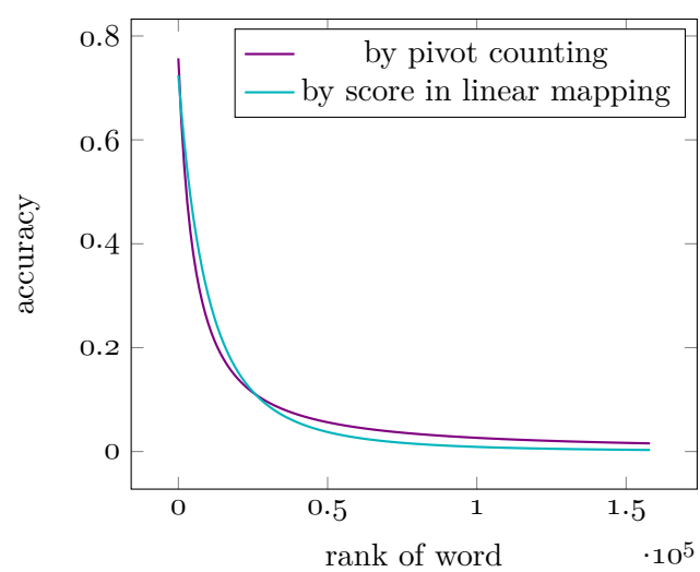
Figure 28: The power law approximations of the accuracy curves.
