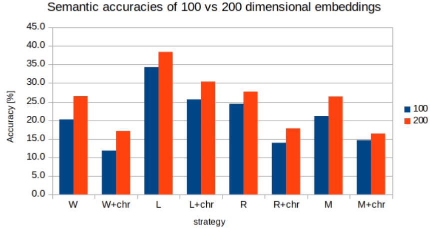
Figure 12: Semantic accuracy of Hungarian 100 and 200 dimensional embeddings with different strategies; context window covers 21 units.
