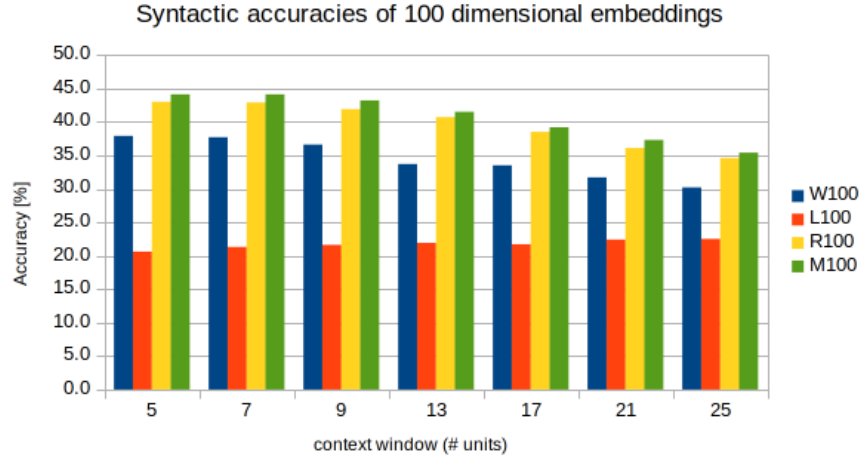
Figure 10: Syntactic accuracy of Hungarian 100 dimensional embeddings with different strategies.
