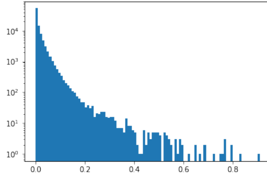
Figure 17: The histogram of the verb embedding matrix elements. Note that the vertical axis, which corresponds to the histogram count in each bin, is logarithmic. The figure suggests that frequency decreases faster than exponentially as larger weights are considered.
